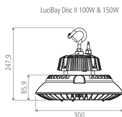
Lucibay Disc II 100W &amp; 150W
