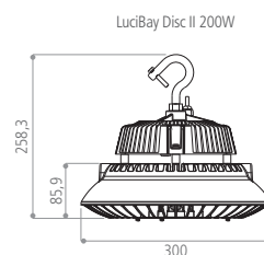
Lucibay Disc II 200W
